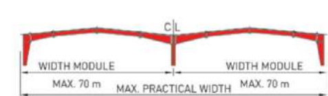
Multi Gable
