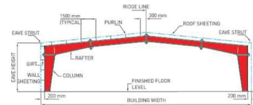
Frame Cross Section
