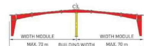
Multi Span
