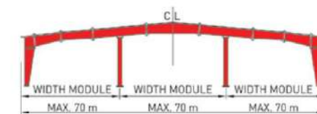
Multi Span
