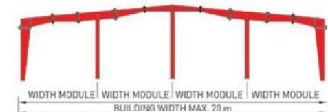
Multi Span
