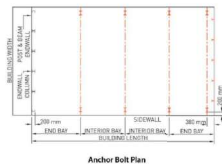
Anchor Bolt Plan
